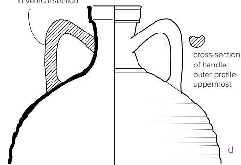
Two-handled vessel: left-hand handle shown in vertical section
